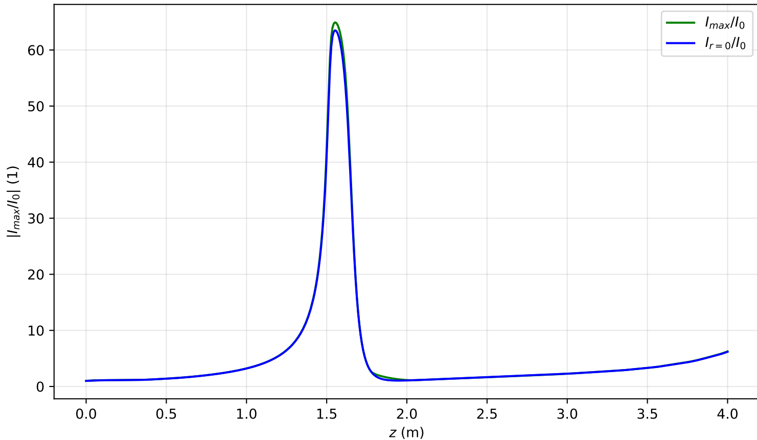
I_{max}(x=0, y=0, z)/I_0 , \text{Pin}=1.6\text{Pcr} , noisy input, artificial time
